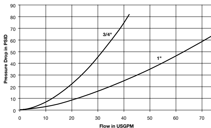
4000 Series (3/4" & 1") Test Fluid: Oil - 200 SUS
